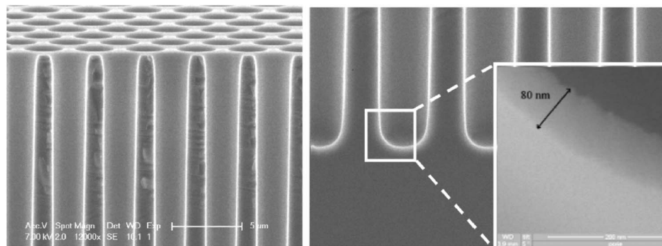
Figure 6. High-resolution SEM images of Al_2O_3 deposited by remote plasma ALD in macropore structures with an aspect ratio of \sim 8 (diam: 2–2.5 \mu\text{m} , depth: 19 \mu\text{m} ). The Al_2O_3 was deposited using 700 ALD cycles.
