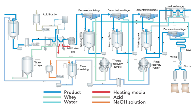
Fig. 1. Casein production process (TetraPack, 2015).
