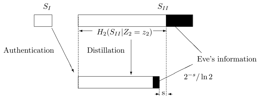
Figure 3.4: Privacy amplification with a totally secret authentication key
