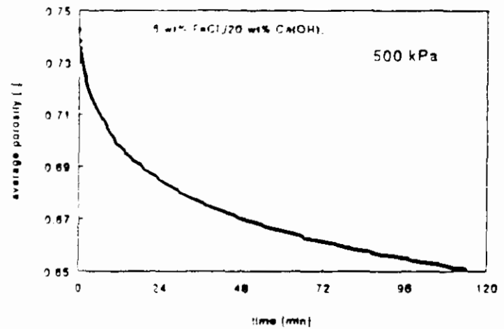
Figure 4. Average porosity versus time, expression experiment (sludge flocculated with 6 wt% \text{FeCl}_3 , and 20 wt% \text{Ca(OH)}_2 , on dry solids basis; \Delta p=500 kPa).
