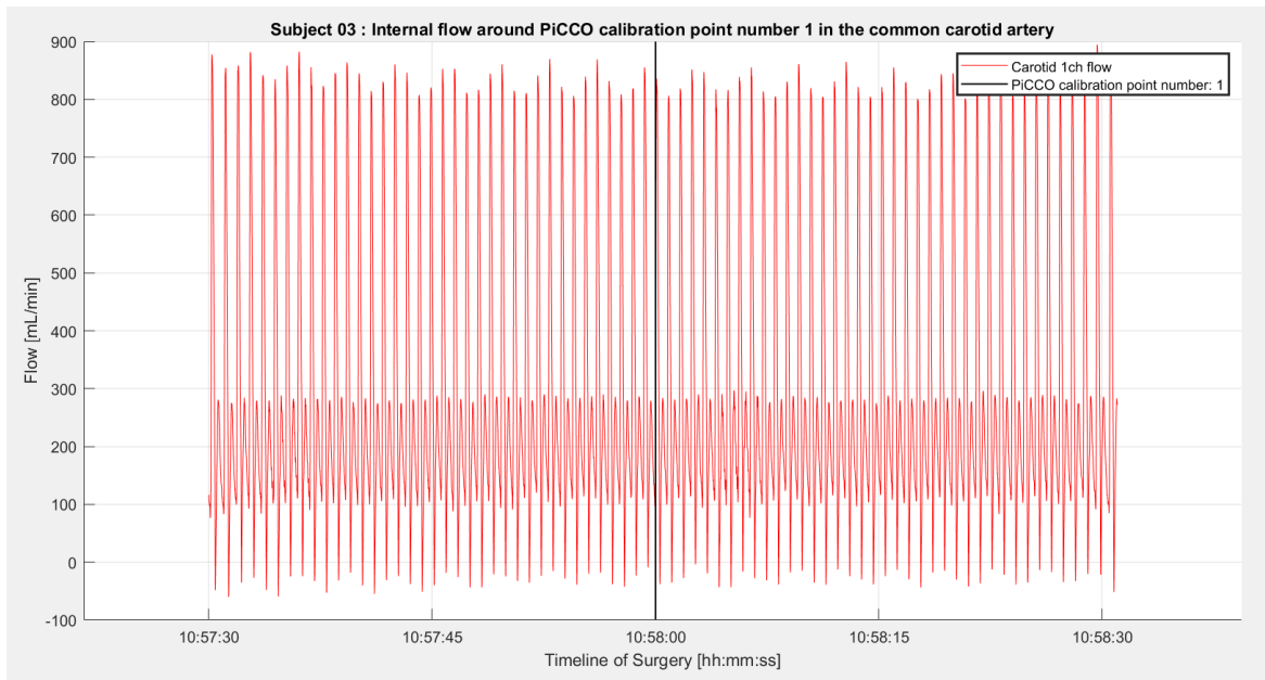
Figure 9. Example of the VFR sensor signal in the common carotid artery measured from Subject 3 at PiCCO calibration point 1.
