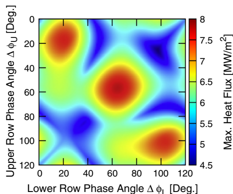
Fig. 3. Maximum heat flux on the upper wall as a function of the phase angles.
