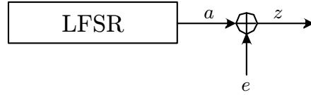
Figure 4.1: Statistical model of a combination generator
