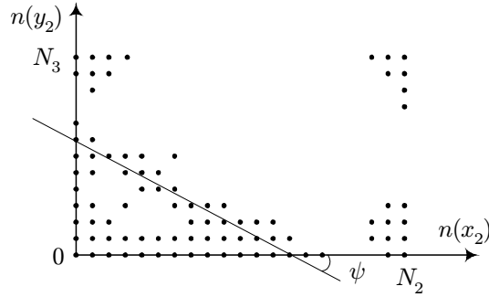
Figure 4.3: The sample space when N_4 = 0
