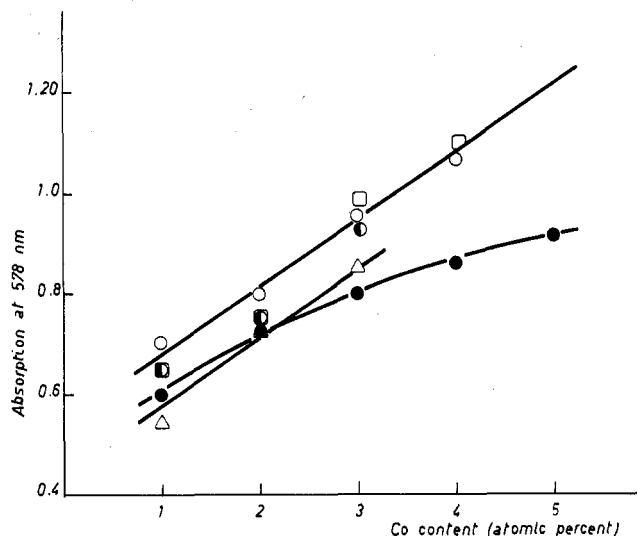
Figure 3. Intensity of the absorption band at 578 nm vs. cobalt content (atom percent): ( \Delta ) A\gamma\text{Co}_x ; ( \circ ) A\gamma\text{GaCo}(0.6:x) ; ( \bullet ) B-A\gamma\text{GaMoCo}(0.6:5:x) ; ( \square ) A\gamma\text{GaCo}(4:x) ; ( \bullet ) A-A\gamma\text{GaMoCo}(0.6:5:x) .
