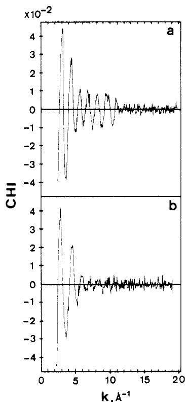
Figure 3. The normalized EXAFS oscillations \chi(k) vs. k (measured at 140 K): (a) reduced catalyst (100 kPa \text{H}_2 ); (b) CO adsorbed catalyst (100 kPa CO).
