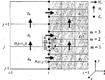
Figure 7: Coarse-fine grid interface, refinement factor ( n_{\text{fact}} ) is three (from [17]).
