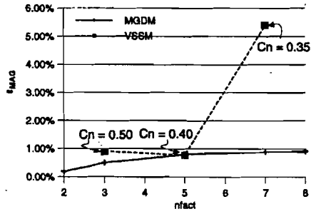
Figure 3: Comparison between magnitude errors ( \varrho_{MAG} ) of the electric field as calculated by MGDM and VSSM. The size of the regions were 4 \times 4 \times 4 fine grid cells (left) and 8 \times 8 \times 8 fine grid cells (right). Courant number of 0.57 was used in MGDM (from [16]).
