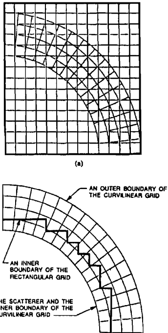
Figure 8: Combination of the cartesian and the curvilinear grid (top), inner boundary of the rectangular grid (bottom) (from [19]).
