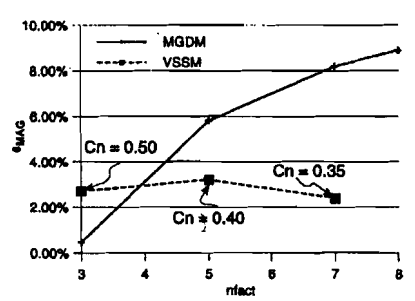
Figure 3: Comparison between magnitude errors ( \epsilon_{MAG} ) of the electric field as calculated by MGDM and VSSM. The size of the regions were 4 \times 4 \times 4 fine grid cells (left) and 8 \times 8 \times 8 fine grid cells (right). Courant number of 0.57 was used in MGDM (from [16]).
