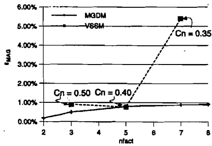
Figure 3: Comparison between magnitude errors ( \epsilon_{MAG} ) of the electric field as calculated by MGDM and VSSM. The size of the regions were 4 \times 4 \times 4 fine grid cells (left) and 8 \times 8 \times 8 fine grid cells (right). Courant number of 0.57 was used in MGDM (from [16]).
