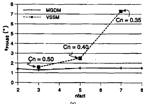
Figure 4: Comparison between phase errors ( \varrho_{PHASE} ) of the electric field as calculated by MGDM and VSSM. The size of the regions were 4 \times 4 \times 4 fine grid cells (left) and 8 \times 8 \times 8 fine grid cells (right). Courant number of 0.57 was used in MGDM (from [16]).
