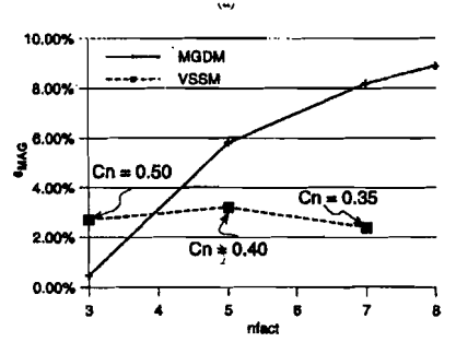
Figure 3: Comparison between magnitude errors ( \varrho_{MAG} ) of the electric field as calculated by MGDM and VSSM. The size of the regions were 4 \times 4 \times 4 fine grid cells (left) and 8 \times 8 \times 8 fine grid cells (right). Courant number of 0.57 was used in MGDM (from [16]).
