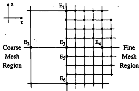
Figure 2: Regions used to calculate fields at the coarse/fine grid interface (from [12])
