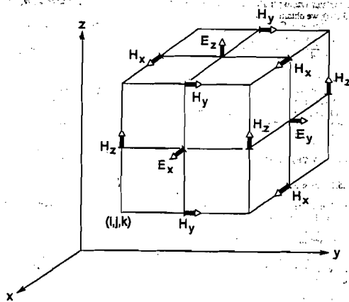
Figure 1: Yee cell
