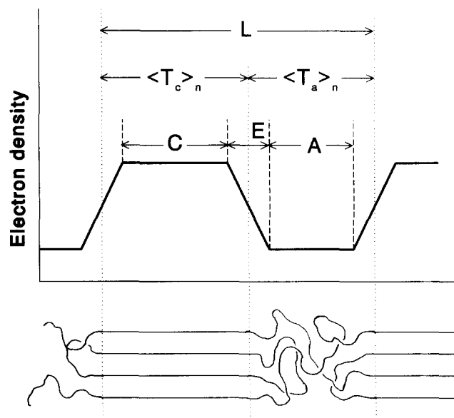
Figure 1 Schematic presentation of the lamellar morphology, perpendicular to the lamellae, and the corresponding electron density profile according to the pseudo-two-phase model described by Vonk 16 : L = periodicity, \langle T_c \rangle_n = lamellar thickness, \langle T_a \rangle_n = amorphous thickness, C = lamellar core, A = amorphous core, E = transition layer
