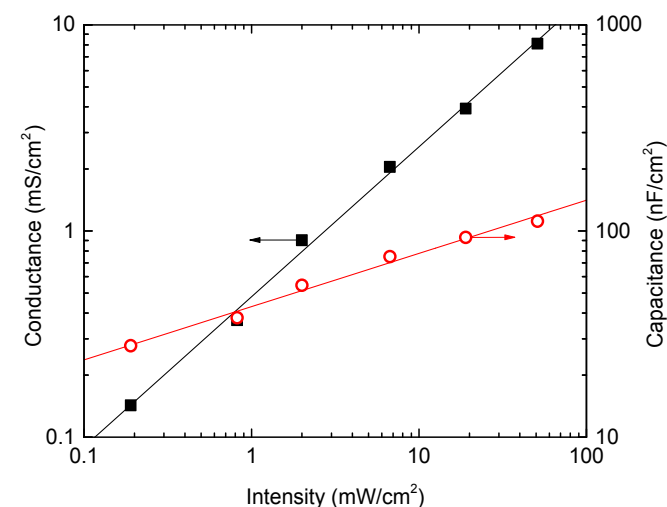
Fig. 2. The parallel conductance (black squares) and parallel capacitance (red open circles) as function of illumination intensity at a frequency of 1000 Hz and a dc bias voltage equal to the open circuit voltage. Solid lines show the fit of a power law function to the data with exponents 0.73 \pm 0.02 (conductance, black line) 0.26 \pm 0.01 (capacitance, red line). (For interpretation of the references to colour in this figure legend, the reader is referred to the web version of this article.)
