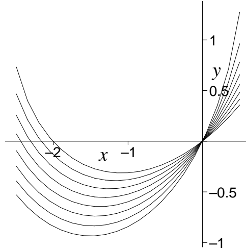
FIGURE 1. Some integral curves of the o.d.e.
