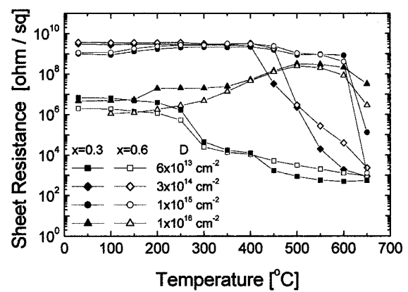
FIG. 2. Thermal stability of the proton beam isolated layers of n -type \text{Al}_x\text{Ga}_{1-x}\text{As} with x=0.3 and x=0.6 , irradiated to different doses D .
