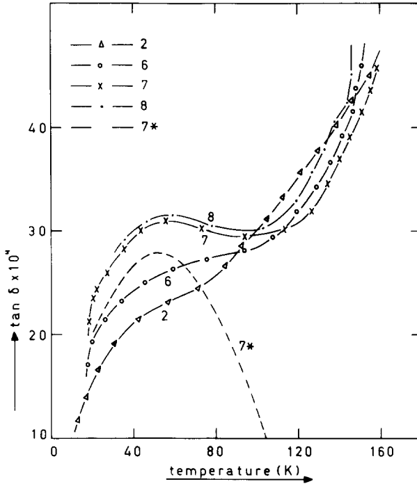
Fig. 1. Dielectric loss curves for sodium phosphate glasses. Sample 2, Na 2 OP 2 O 5 ; samples 6, 7 and the same 8 with the addition of cyclic trimetaphosphate (cf. tables 1 and 2). Curve 7* shows the peak of sample 7 after the subtraction of the exponential background due to the migration loss peak.
