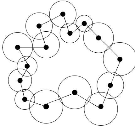
FIG. 4. The necklace TSP.
