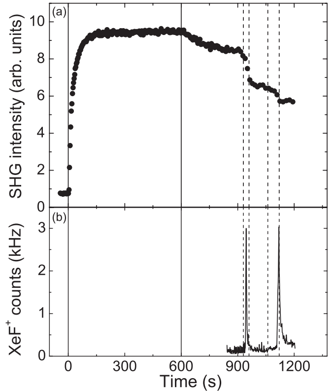
FIG. 7. (a) Real time SHG response of H terminated Si(100) (closed circles) bombarded with 70 eV \text{Ar}^+ ions at a flux of \sim 0.07 ML/s followed by two small doses of \text{XeF}_2 (in total \sim 30 ML). Between t=0 s and t=600 s the sample is exposed to ion bombardment. Between t=930 s and t=960 s and between t=1060 s and t=1120 s the \text{XeF}_2 beam is switched on. The SH photon energy is 3.31 eV and both the fundamental and the SH radiation are p polarized. (b) The count rate due to \text{XeF}^+ as measured with the quadrupole mass spectrometer (QMS) during dosing.
