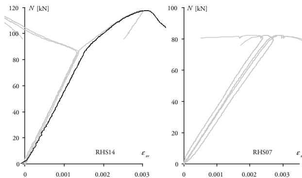
Figure 11: Characteristic load-strain curves: (strain gauges in grey, LVDT in black)
