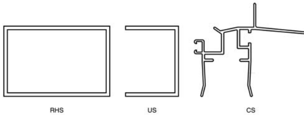
Figure 5: Examples of cross-sections tested in the Eindhoven program
