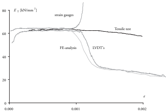
Figure 16: Comparison of the tangent stiffnesses of the compression test (strain gauges and LVDT's), tensile test and FE-analysis (CS11-2)
