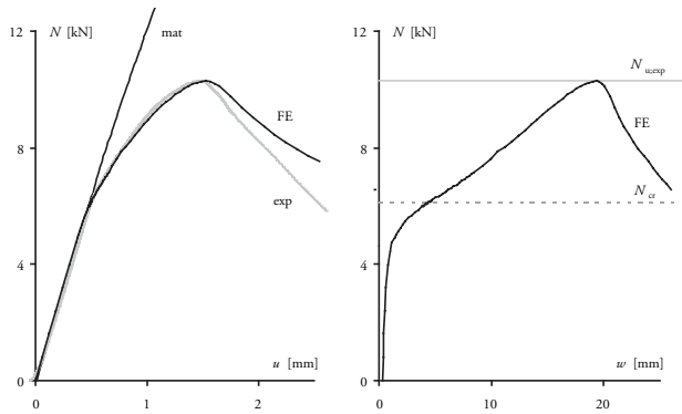
Figure 15: Experimental and numerical load-displacement and load-deflection curves (CS11-2)
