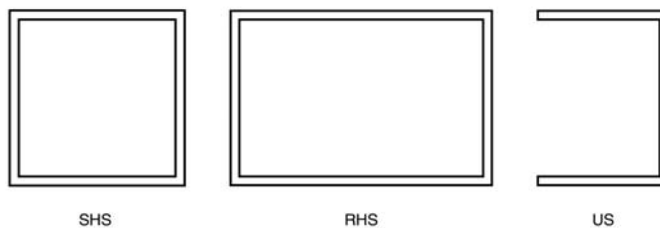
Figure 3: Cross-sections tested in the Salerno program
