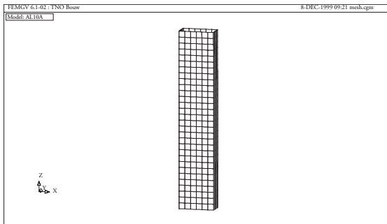
Figure 12: Mesh schematisation of specimen RHS10
