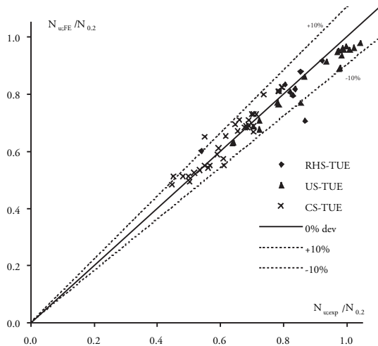
Figure 17: Comparison of experimental and FE-results – Ultimate loads
