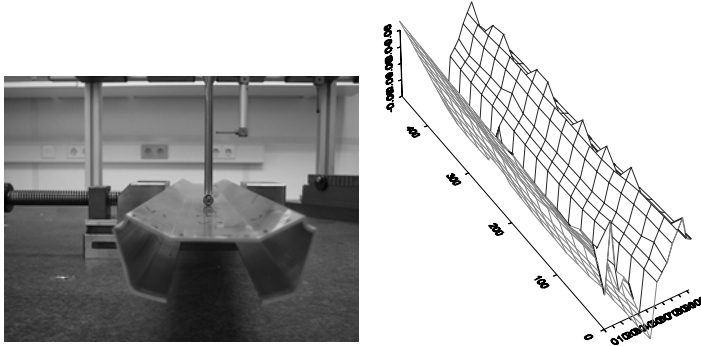
Figure 8: Set-up and characteristic results of imperfection measurements – Specimen CS05
