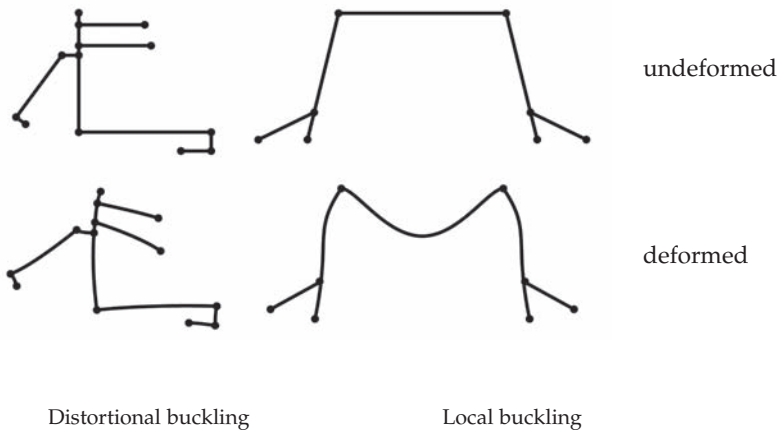
Figure 2: Cross-sectional instability – Local and distortional buckling
