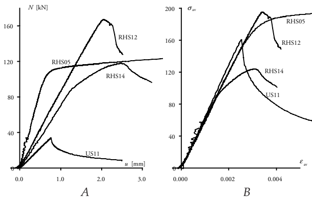
Figure 10: Characteristic load-displacement and stress-strain diagrams, Eindhoven program
