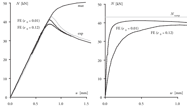
Figure 14: Experimental and numerical load-displacement and load-deflection curves (US10)
