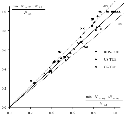
Figure 18: Comparison of experimental and FE-results – Bifurcation loads
