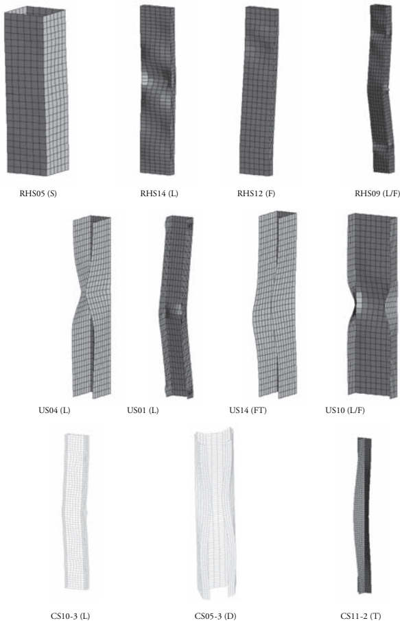
Figure 13: Deformations at failure – FE-results
