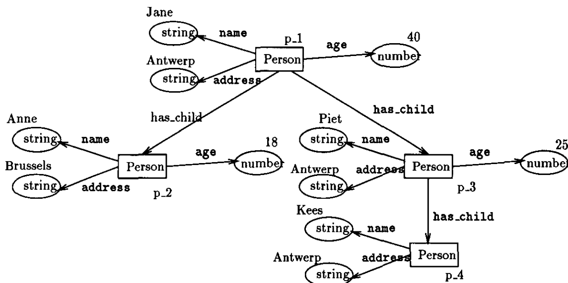
Figure 1: A simple instance
