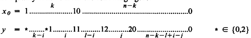
FIGURE 1. Two words having L -distance d_L(x_0, y) = k + l - 2i + 2j .
