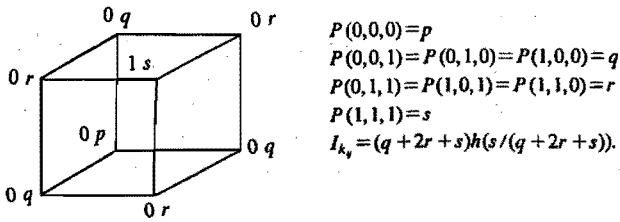
FIGURE 3. Probabilities and output symbols to obtain the maximal value for I_3^{12} + I_2^{13} + I_1^{23} .
