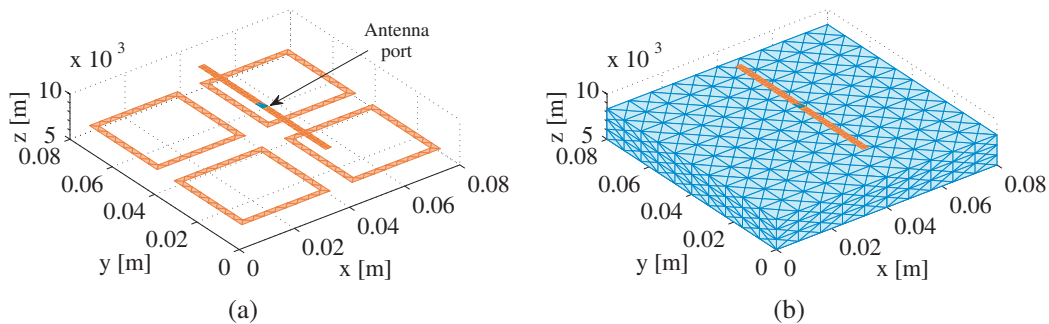
Figure 1. Simple radiation problem: (a) A strip-dipole in the presence of four square loops; (b) Corresponding LEGO model with N_D = 4 cuboidal bricks.
