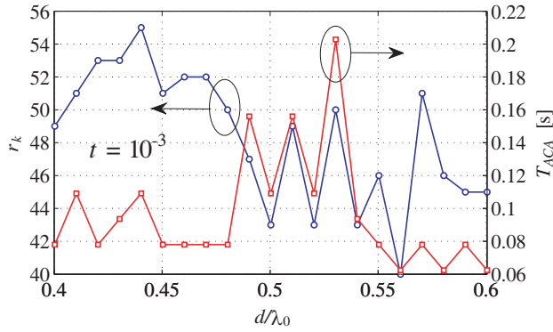
Figure 4. ACA decomposition (threshold t ) of [S_{kk}] for the bricks used to model the antenna system in Fig. 1: (○) effective rank of [S_{kk}] and (□) CPU time versus the electric length of the strip-dipole.
