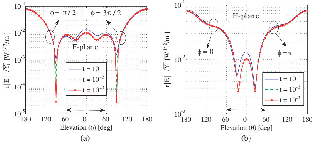
Figure 3. Convergence of solutions with ACA macro basis functions: normalized magnitude of the total electric field radiated by the antenna system in Fig. 1; (a) E -plane ( yOz ); (b) H -plane ( xOz ). The parameter ( t ) of the lines is the threshold used in (9).
