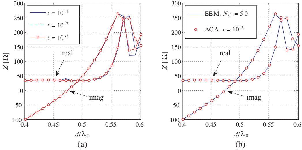
Figure 2. Input impedance of the antenna system in Fig. 1 as a function of the electric length of the strip-dipole: (a) Convergence with increasing number of ACA macro basis functions; (b) Comparison with the results obtained through the eigencurrents expansion method (EEM) [24].
