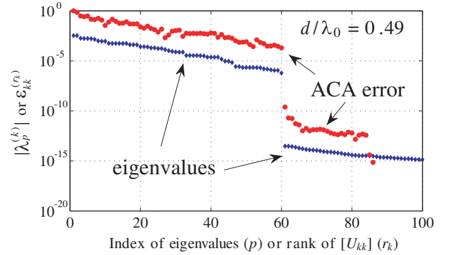
Figure 5. Low-rank nature of [S_{kk}] for the bricks used to model the antenna system in Fig. 1: (◆) eigenvalues of [S_{kk}] versus their index; (●) relative error of the ACA decomposition of [S_{kk}] versus the rank of [U_{kk}] .
