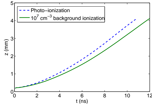
Figure 7. Position of streamer head as a function of time for two cases in N_2 with 1ppm O_2 . Solid curve: 10^7 \text{ cm}^{-3} background ionization, no photo-ionization. Dashed curve: photo-ionization, no background ionization. The gap between the electrodes is 8 mm and the potential is 20 kV. For both cases, the available data was limited by the fact that branching occurs at around 4 mm and the simulations were halted before the streamers reached the cathode.
