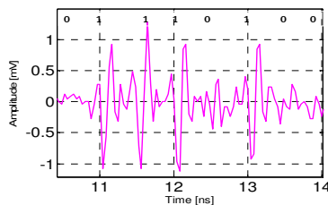
Fig. 3a: IR-UWB in optical back-to-back case
