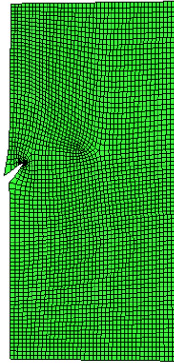
Figure 5 - a) Deformed initial plate.
