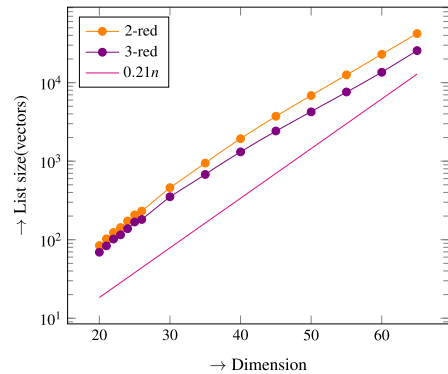
(b) List sizes for dimensions 20–65.
