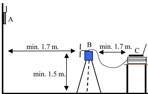
Fig. 5 Measured set up. A: WLAN router. B: Measurement antenna on tripod. C: Spectrum analyser and computer for data storage and processing.
