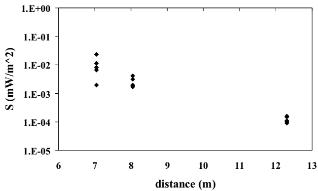
Fig. 9 Measured WLAN peak power density levels as a function of distance to the nearest WLAN router.
