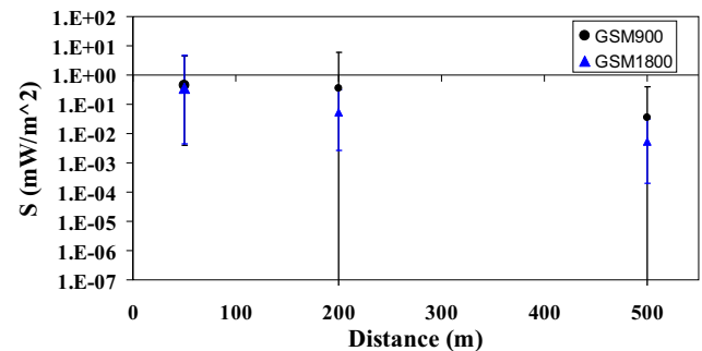
Fig. 4 Measured summed power density levels as a function of distance to the nearest GSM-900 and GSM-1800 base station. Data is taken from [8].
