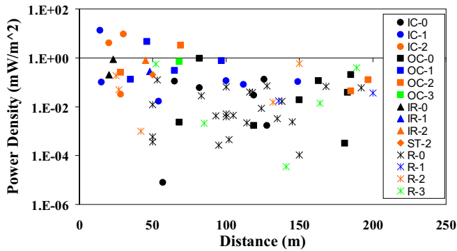
Fig. 1 Measured GSM-900 peak power density levels as a function of distance to the nearest base station. Data is taken from [5]. Code 'XY-a' indicates area and measurement site characteristics. XY: IC=Inner City, OC=Outer Country, IR=Industrial area, ST=Small Town, R=Rural or country-side are. a: 0=outdoors on the ground, 1=outdoors on roof, terrace or balcony, 2=indoors, close to windows, 1.5m or less, 3=indoors, not close to windows.
