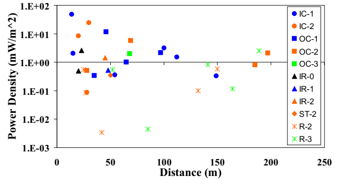
Fig. 3 Measured GSM-900 summed power density levels as a function of distance to the nearest base station, without data taken on ground level. Data is taken from [5].
