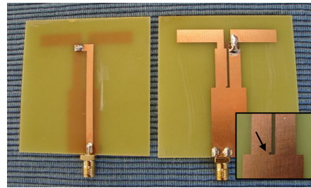
Fig. 6 Realisation on FR4 of a printed dipole antenna with integrated microstrip via-hole balun, back and front. Inset: indication of phase centre.
