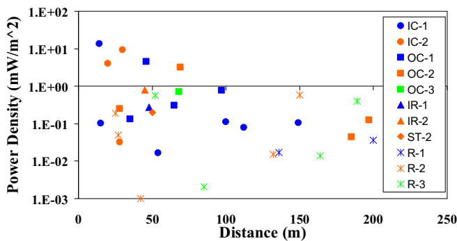
Fig. 2 Measured GSM-900 peak power density levels as a function of distance to the nearest base station. Data is taken from [5]. Same as Figure 1 but with data taken on ground level removed.
