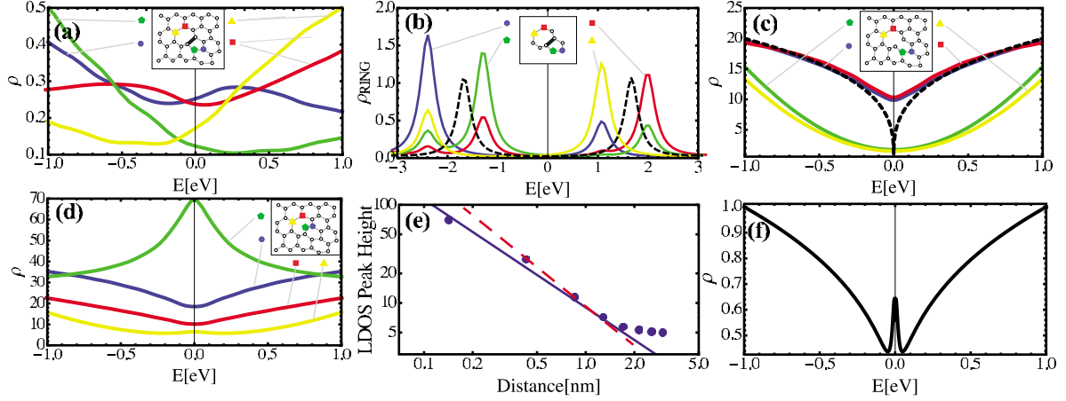
FIG. 1. (Color online) The LDOS of graphene dislocations from tight-binding and continuum theory. (a) LDOS of representative atoms of the PH type dislocation core (inset, see Sec. II A). As discussed in Sec. II B, the weight is shifted due to the A-A bond (thick in the inset), compared to the symmetric curves in (c) obtained by switching off the A-A bond that are consistent with continuum theory. (b) The influence of the A-A bond on an isolated ring: the lattice case (a) can be viewed as a broadened version. (c) PH core LDOS without the AA bond. Dislocation topology effects from continuum theory (Sec. II B, dashed black curve) are prominent. (Finite LDOS at E=0 is a finite-size effect.) (d) LDOS of representative atoms in OCT core type. (e) The height of LDOS peak in (d) (pentagon, green) falls off like a power law with distance from defect core. Red (dashed) line is the continuum theory prediction for a zero mode, with exponent -4/3 (see Sec. II C). The power-law behavior holds also for LDOS features in (a). (f) The continuum defect topology prediction of LDOS (in patch of radius \delta=0.1 , Sec. II B) in a dislocation array with zero modes.
