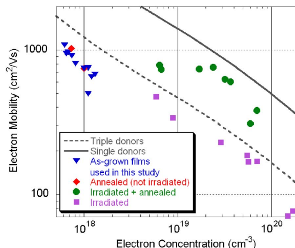
FIG. 1. (Color online) Electrical properties of the films used in this study, as grown and after irradiation and/or thermal annealing treatments. Theoretical \mu limited by singly and triply charged donor defect scattering is also shown. In the irradiated films, the higher n correspond to higher 2 MeV He + fluences.
