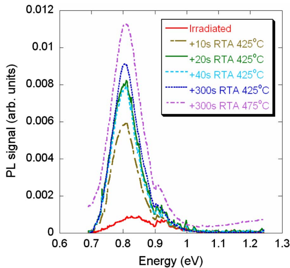
FIG. 2. (Color online) PL signal of one InN film after irradiation with 1.1 \times 10^{15} \text{ He}^+ \text{ cm}^{-2} and then successive thermal annealing treatments.
