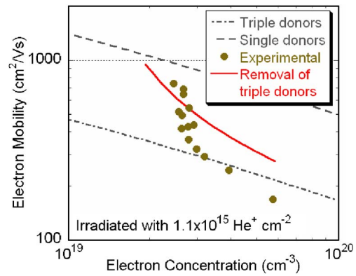
FIG. 3. (Color online) \mu as a function of n in an InN film after each successive thermal annealing treatment. The solid line was calculated by assuming that irradiation produces a 3:2 ratio of singly to triply charged defects, and that the only effect of thermal annealing is to remove triply charged donor defects. The poor correspondence between the model and the experimental data is evidence for spatial ordering of the remaining defects.
