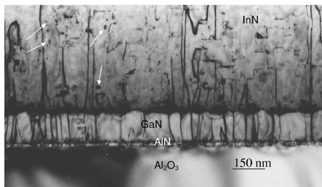
FIG. 4. Cross-section micrograph of one InN film after irradiation with 8.9 \times 10^{15} \text{ He}^+ \text{ cm}^{-2} and then thermal annealing. The concentration of dislocation loops with size between 5 and 20 nm is 9 \times 10^{10} \text{ cm}^{-2} ; as an example, four of the loops are marked by arrows. The AlN/GaN buffer layer and sapphire substrate are also shown.
