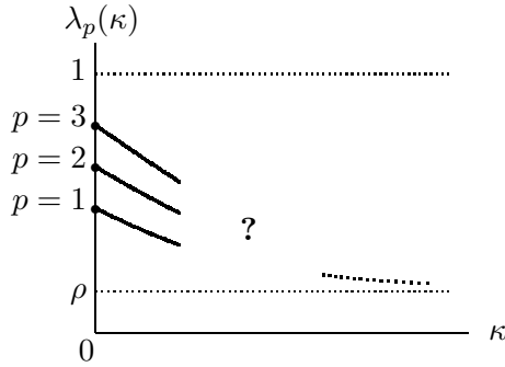
Fig. 3: Qualitative picture of \kappa \mapsto \lambda_p(\kappa) for p = 1, 2, 3 for simple random walk in d \geq 4 . The dotted line moving down represents the asymptotics given by the r.h.s. of (1.3.1).
