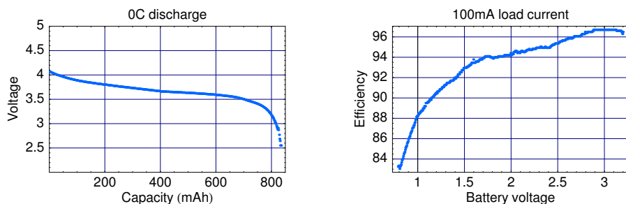
(a) Battery terminal versus state of charge curve for a Panasonic CGR17500 Lithium ion battery [Panasonic, Inc. 2000]. (b) Voltage regulator efficiency curve for a TI TPS61100 voltage regulator [Texas Instruments, Inc. 2002].
