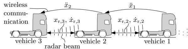
Fig. 1. Schematic representation of a platoon of vehicles equipped with CACC functionality, where x_{r,i} , \hat{x}_{r,i} and \ddot{x}_i represent the relative position, the relative velocity and the acceleration of vehicle i , respectively.
