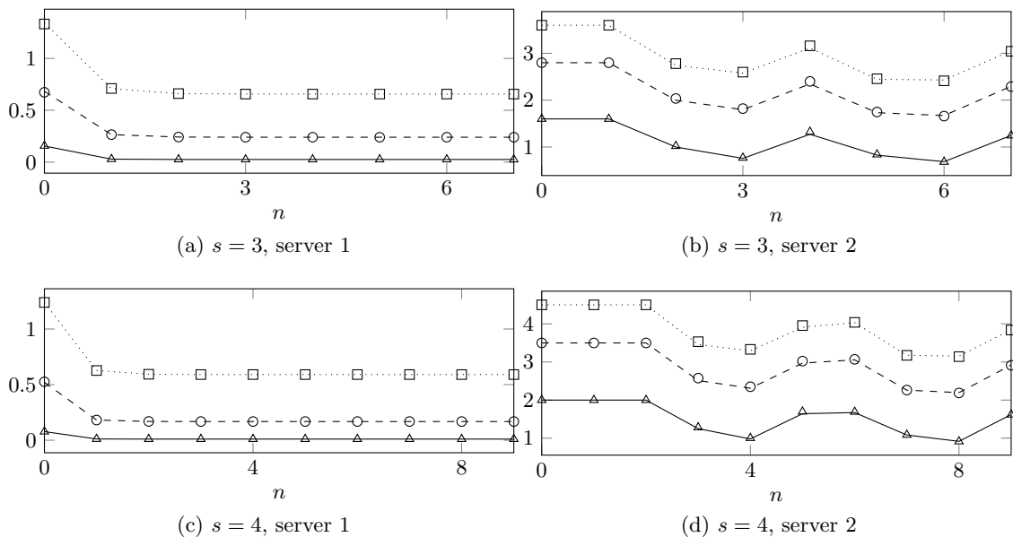
Figure 4: Comparison of conditional arrival rates determined by the algorithm in [14] (lines) and our approximations (marks) for \rho = 0.4 ( -,\Delta ), \rho = 0.7 ( --,\circ ), and \rho = 0.9 ( \cdots,\square ).
