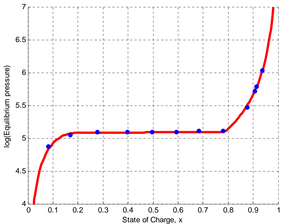
FIG.8. Measured (symbols) and calculated (line) pressure-composition isotherm for the stoichiometric alloy \text{LaNi}_{4.0}\text{Cu}_{1.0} . The measurements have been performed via the gas phase 20\text{ }^\circ\text{C}^{4,19} .
