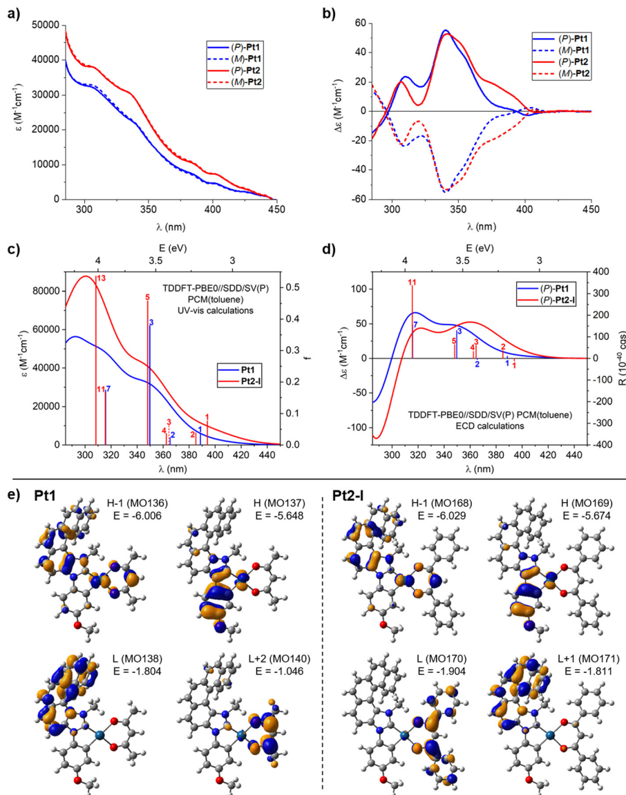
Fig. 2 Experimental (a) UV-visible absorption and (b) ECD spectra of (P)-(+ and (M)-(–) enantiomers of Pt1 and Pt2 measured in toluene at room temperature ( C = 1 \times 10^{-5} M) along with the corresponding TDDFT-simulated spectra (panels (c) and (d), respectively; results for the lowest-energy rotamer (l) of Pt2 shown). (e) Isosurfaces ( \pm 0.04 au) of MOs involved in selected electronic transitions of Pt1 and Pt2. See ESI† for a full set of computed data including the electronic assignment of the spectra.
