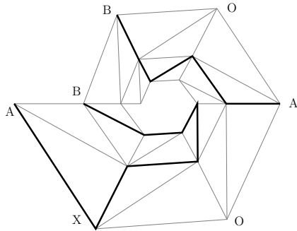
Fig. 2. Partially constructed cycle with signature AXOAOBB
