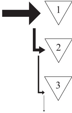
Figure 1: Demand overflow from warehouse 1 when \sigma_1 = (2, 3) .
