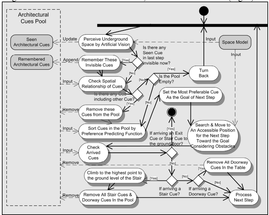
Figure 1. The framework of Architectural Cue Model
