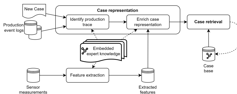
Figure 1: Main steps of the CBR-based decision support for quality incidents.
