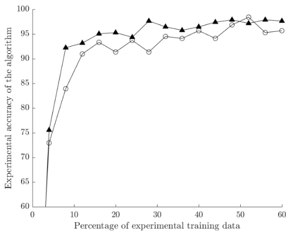
Fig. 6: Accuracy of the optimized SVM (o) and RF ( \Delta ) when classifying experimental data.
