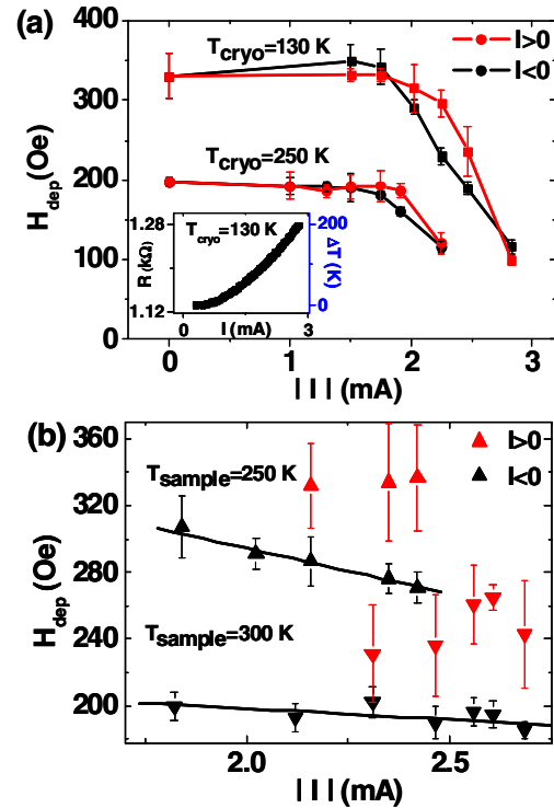
FIG. 2 (color online). (a)–(b) H_{dep} as a function of |I| for (a) a constant cryostat temperature of T_{cryo} = 130 K (squares) and T_{cryo} = 250 K (circles) and (b) a constant sample temperature of T_{sample} = 250 K (up triangles) and T_{sample} = 300 K (down triangles). Each point corresponds to the mean value of H_{dep} averaged over 10 measurements or more and the error bars show the standard deviation. In (b), the black lines are a linear fit of the data. Inset in (a): dependence of the resistance and of the sample temperature rise \Delta T with the current for T_{cryo} = 130 K.
