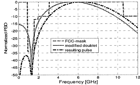
Fig. 2. PSD of the modified doublet, resulting pulse and FCC mask.
