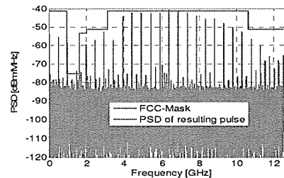
Fig. 6. PSD of proposed pulse versus FCC mask
