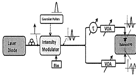
Fig. 3. Experimental setup
