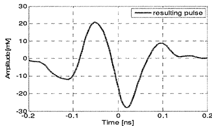
Fig. 5. Proposed UWB-IR pulse shape
