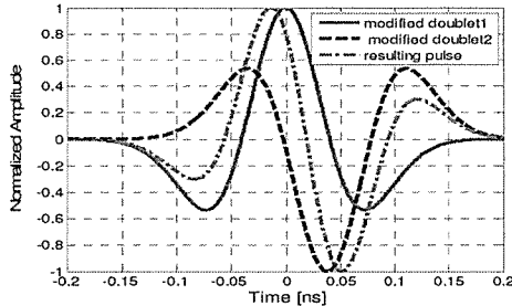
Fig. 1. Modified doublet, its inverted and delayed version, and the resulting pulse.
