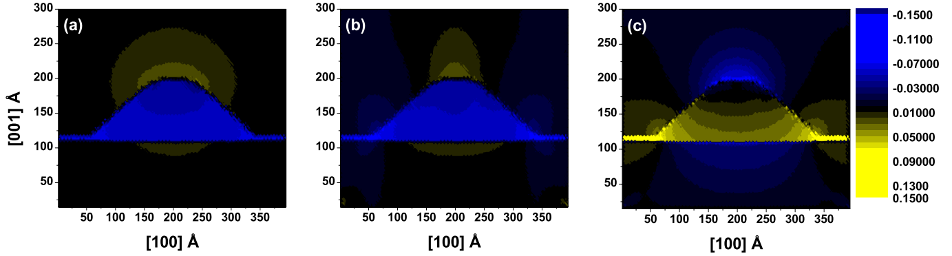
FIG. 9. (Color online) Strain maps for a GaAs/InAs/GaAs quantum dot island. (a), (b), and (c) are the components of the strain \epsilon_{xx} , \epsilon_{yy} , and \epsilon_{zz} .
