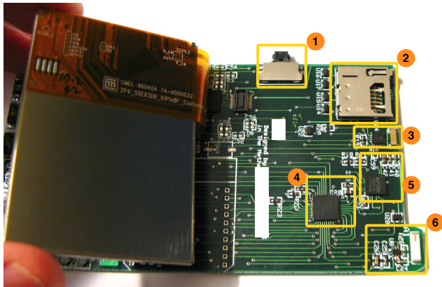
Figure 3. Underside of Sunflower Mobile Client display, showing: (1) the thumb input interface, (2) the microSD card slot, (3) the real-time clock IC and crystal, (4) the system controller, (5) the USB interface IC, and (6) the low-power receive signal strength indication (RSSI) circuit.
