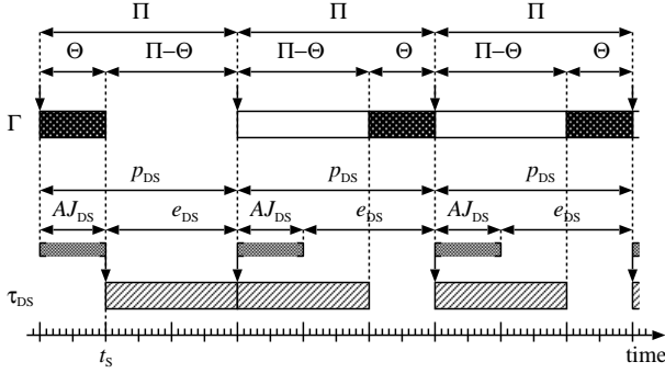
Figure 1. A situation with a worst-case (i.e. minimum) resource supply of a periodic resource \Gamma in an interval starting at time t_s , and a task \tau_{DS} modeling the unavailability of the periodic resource \Gamma .
