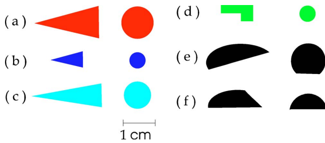
FIG. 4. Particles that display axial drift in rigid-body rotation. Side view (left) and top view (right). The legends in Figs. 5–8 refer to the letters in this figure.
