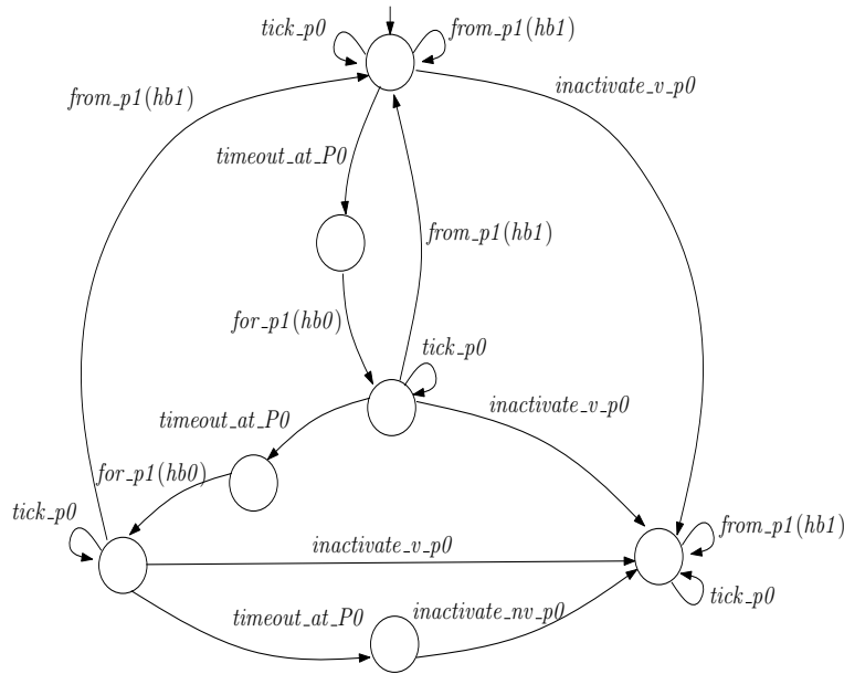
Figure 1: Reduced transition system for process p[0] with tmax=2 and tmin=1
