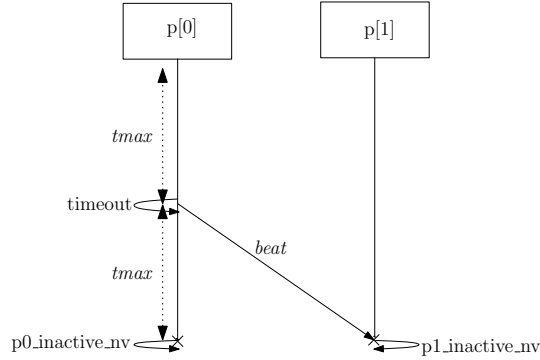
Figure 11: Counter-example for (R2) when t_{min} = t_{max}
