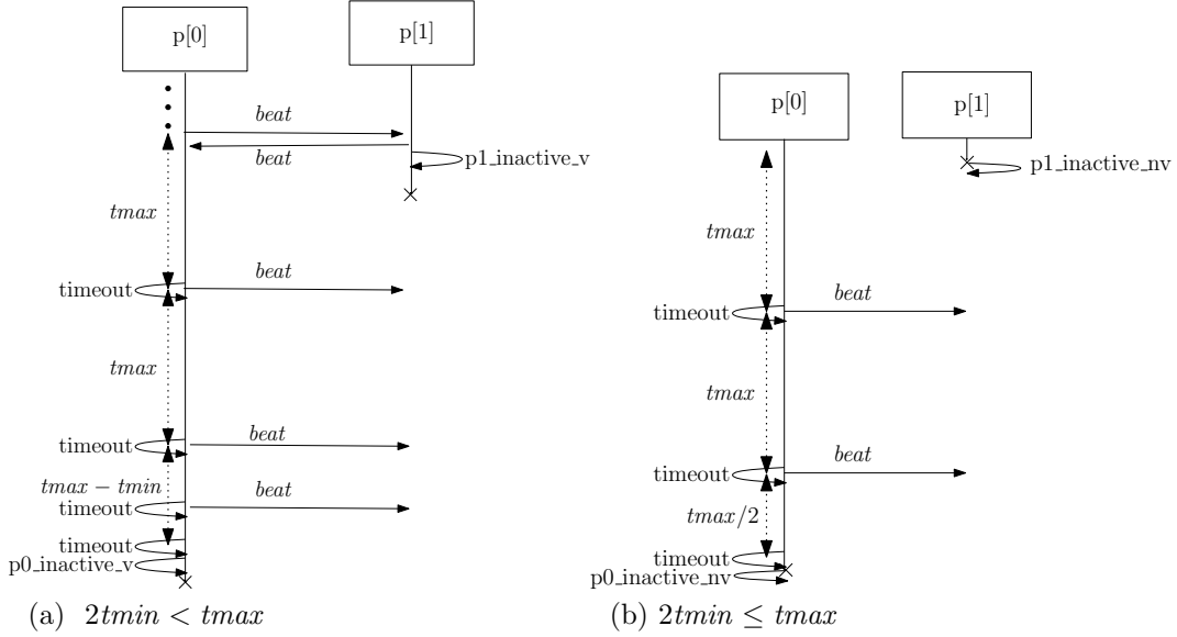
Figure 10: Counter-examples for (R1) when 2t_{min} \leq t_{max}
