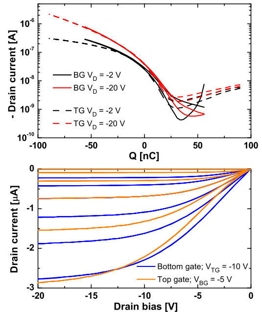
FIG. 3. (Color online) (a) The drain current of the transistor is plotted vs the accumulated charge ( Q ) for both the bottom (solid line) and top (dashed line) gate. For the linear regime, at -2 V (the two lower curves) drain bias, the top gate yields a lower current than the bottom gate for the same induced charge. In the saturated regime, at -20 V (upper curves), both gates show the same current for equivalent charge. (b) Output curves of the top and bottom gate. For both gates, the gate voltage was varied in 5 V steps from 5 V to -20 V. For the top gate drain sweeps, the bottom gate bias was at -5 V and for the bottom gate drain sweeps the top gate bias was -10 V. The output curves for both gates are presented for similar drain currents by tuning the opposing gate's bias, to ease comparing the two measurements.
