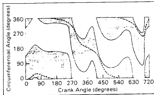
Fig. 13 Pressure curve extent plot for the bearing as obtained from the FEM analysis (full extent). \square P = 0 , \blacksquare P > 0 , - - - Location of P_{max} .
