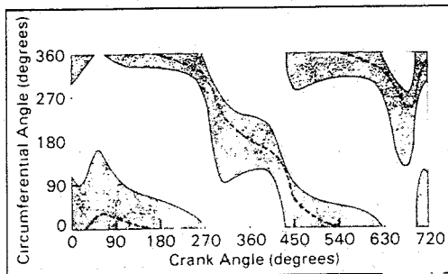
Fig. 12 Pressure curve extent plot for the bearing as obtained from the new curve fit (partial extent). \square P < 0.01 P_{max} , \blacksquare P \geq 0.01 P_{max} , - - - Location of P_{max} .
