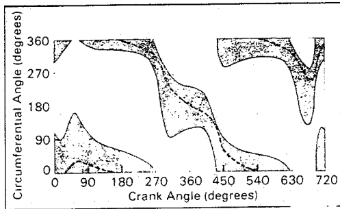
Fig. 12 Pressure curve extent plot for the bearing as obtained from the new curve fit (partial extent). □ P < 0.01 P_{max} , ■ P \geq 0.01 P_{max} , - - - Location of P_{max} .
