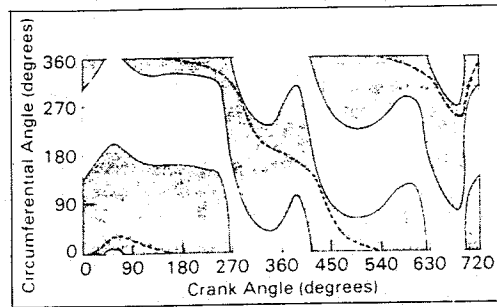
Fig. 13 Pressure curve extent plot for the bearing as obtained from the FEM analysis (full extent). □ P = 0 , ■ P > 0 , - - - Location of P_{max} .
