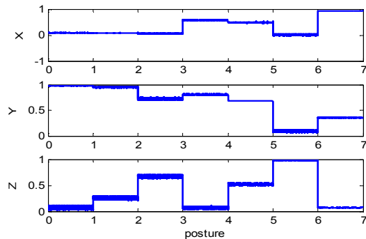
Fig.5. The simulated signals of seven postures, which are represented as seven segments in the plot.
