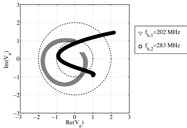
Figure 9. 1000 normalized samples V_n and Chebychev circles C_1 and C_2 .
